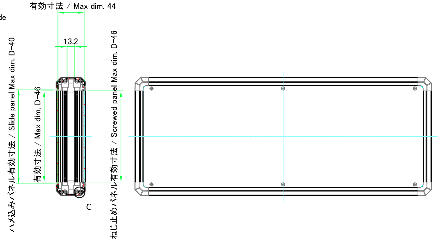
B-B (1:4)
